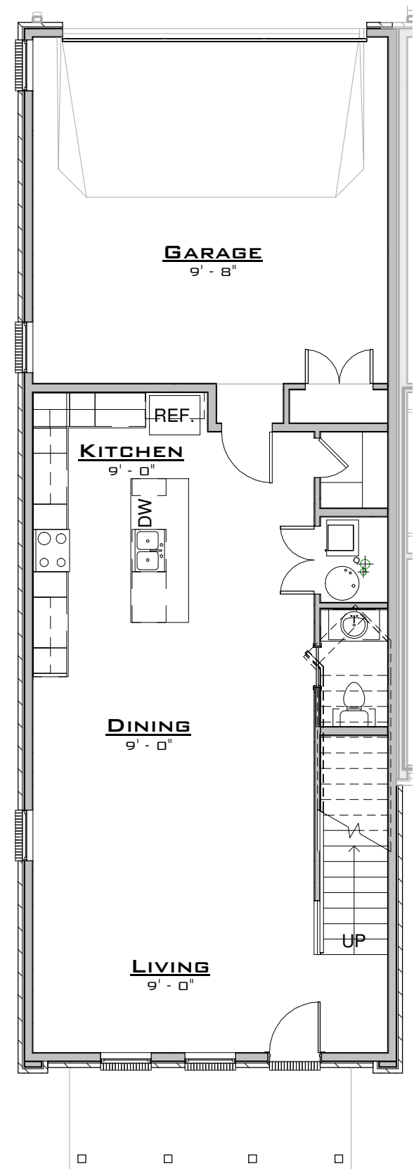
1 FIRST 1/8" = 1'-0"
