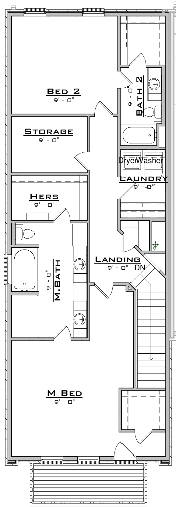
2 SECOND 1/8" = 1'-0"
